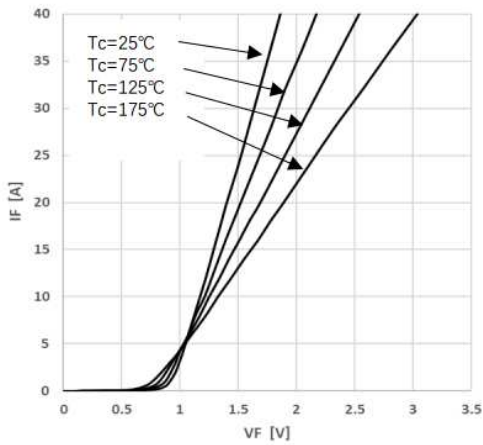
Figure 1 Forward Characteristics
