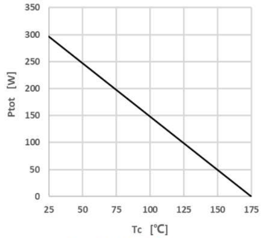
Figure 4 Power Dissipation
