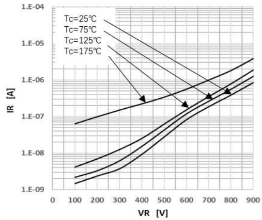
Figure 2 Reverse Characteristics
