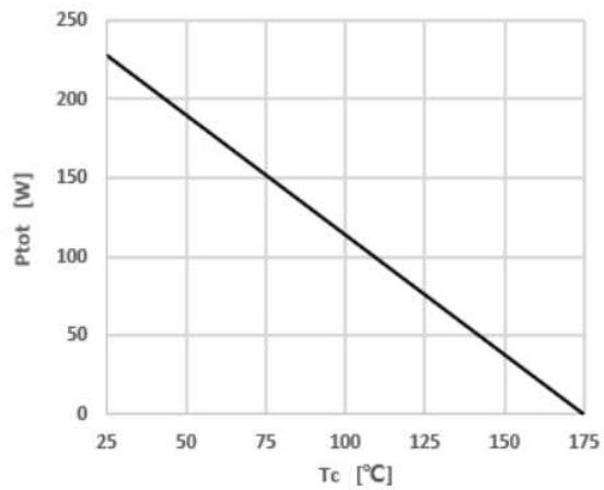
Figure 4 Power Dissipation
