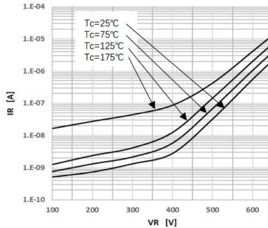
Figure 2 Reverse Characteristics
