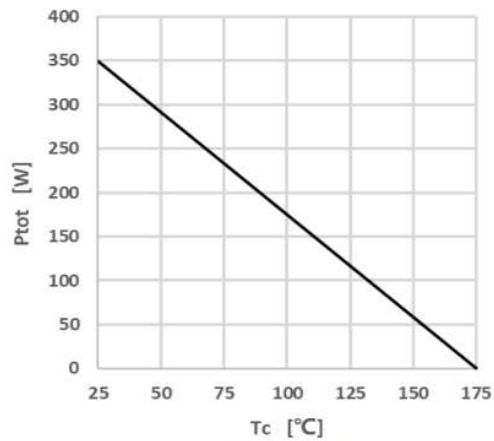
Figure 4 Power Dissipation
