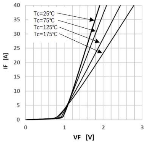
Figure 1 Forward Characteristics
