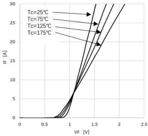
Figure 1 Forward Characteristics
