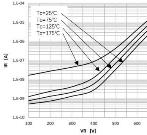
Figure 2 Reverse Characteristics
