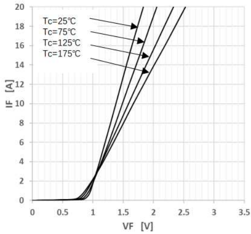
Figure 1 Forward Characteristics
