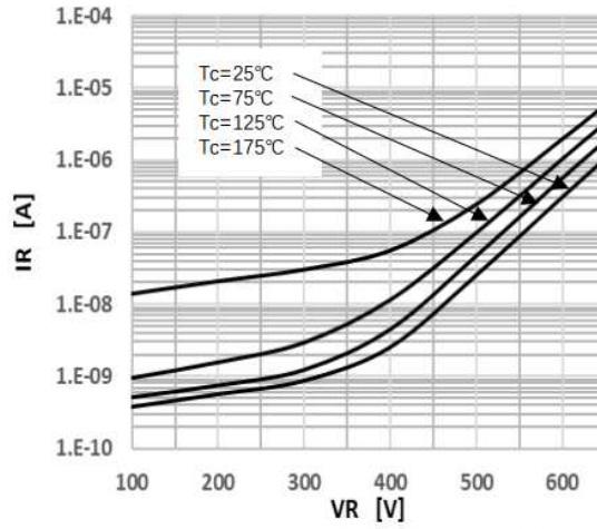
Figure 2 Reverse Characteristics
