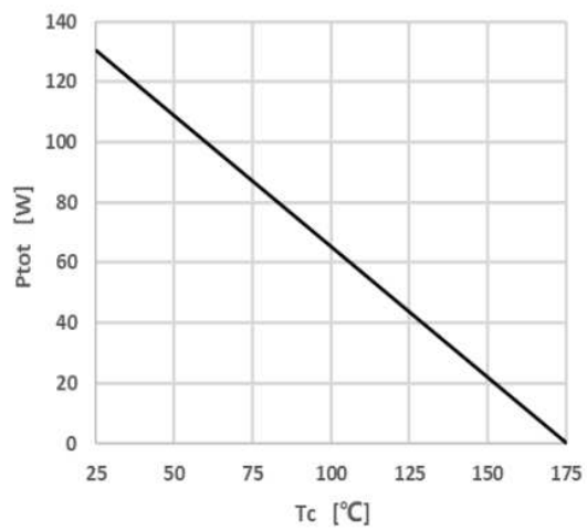
Figure 4 Power Dissipation
