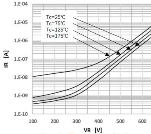
Figure 2 Reverse Characteristics
