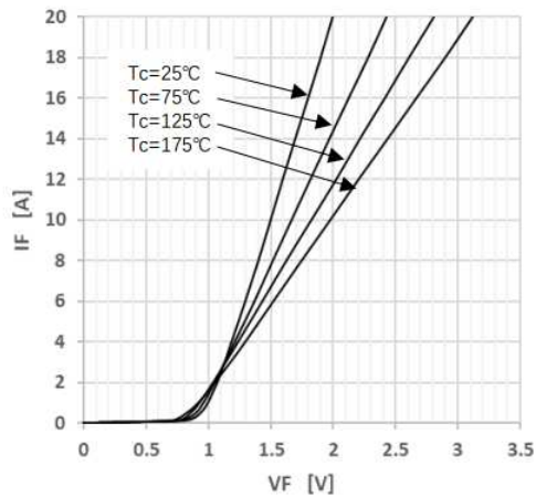
Figure 1 Forward Characteristics
