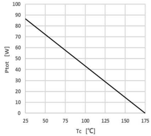
Figure 4 Power Dissipation
