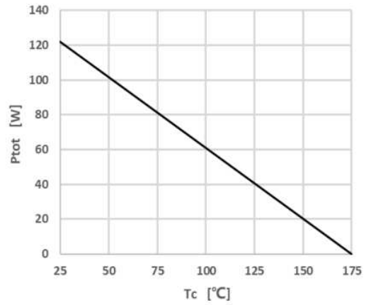
Figure 4 Power Dissipation
