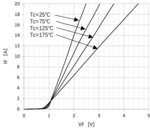
Figure 1 Forward Characteristics
