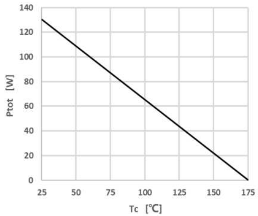
Figure 4 Power Dissipation
