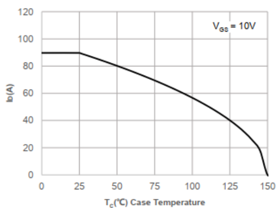
Figure 2. Current De-rating
