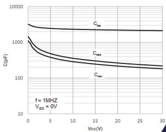
Figure 10. Capacitance Characteristics
