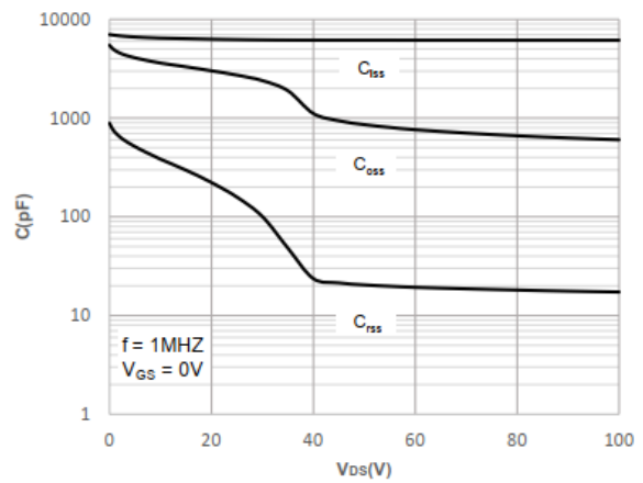
Figure 10. Capacitance Characteristics
