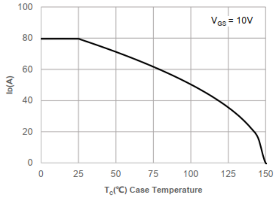
Figure 2. Current De-rating
