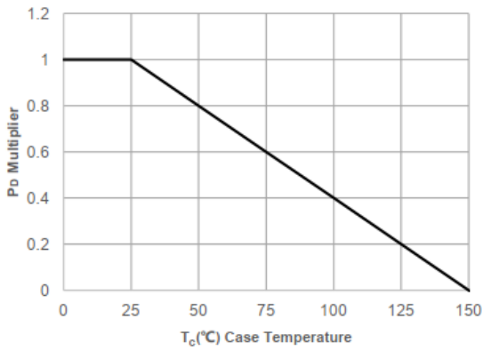
Figure 1. Power De-rating
