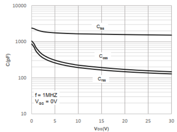
Figure 10. Capacitance Characteristics
