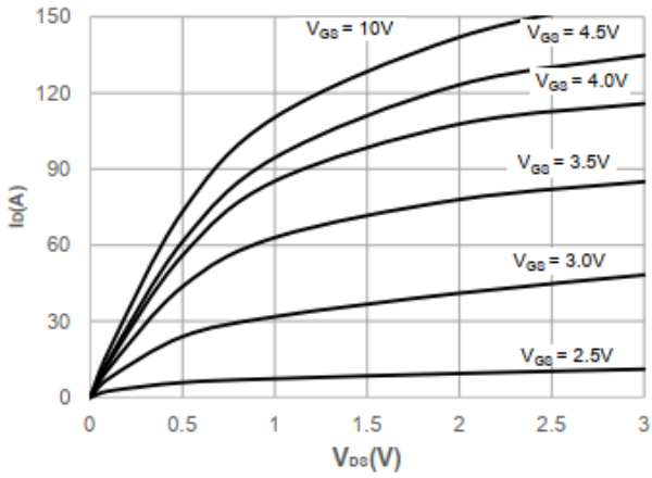
Figure 5. Output Characteristics
