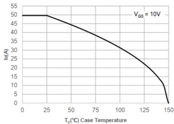
Figure 2. Current De-rating
