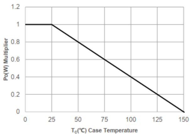
Figure 1. Power De-rating
