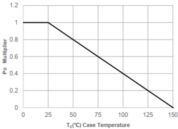
Figure 1. Power De-rating
