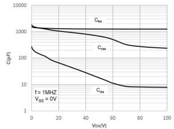
Figure 10. Capacitance Characteristics
