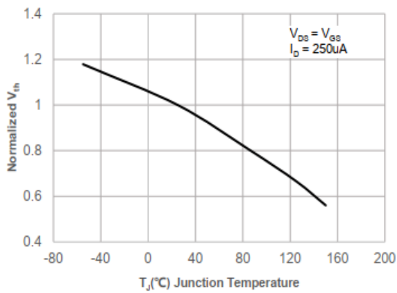
Figure 13. Normalized Threshold Voltage vs. Junction Temperature
