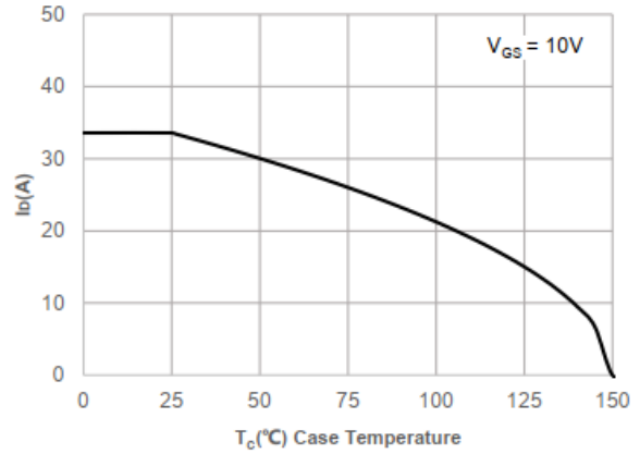
Figure 2. Current De-rating
