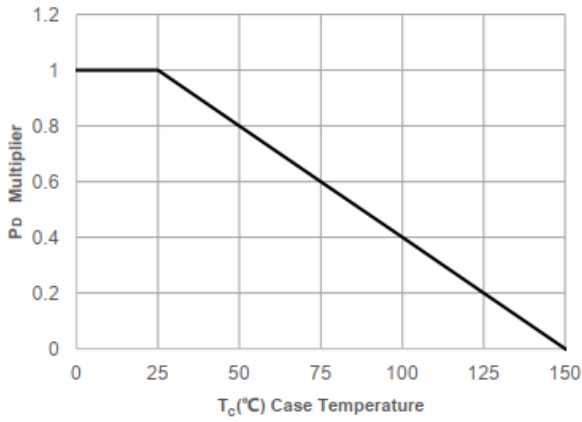
Figure 1. Power De-rating
