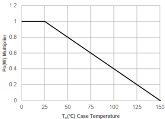
Figure 1. Power De-rating
