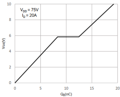
Figure 9. Gate Charge Characteristics
