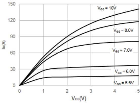
Figure 5. Output Characteristics
