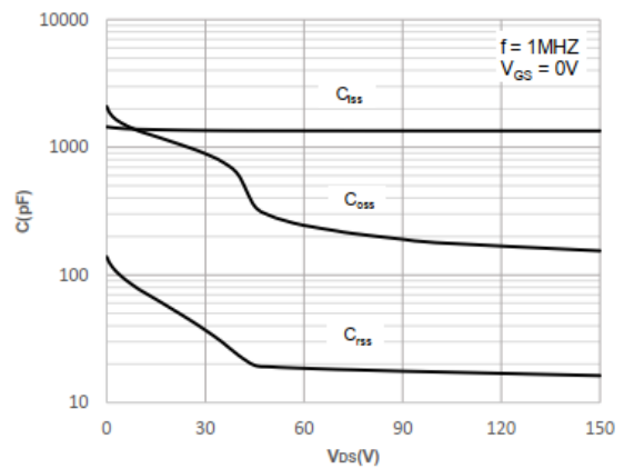
Figure 10. Capacitance Characteristics
