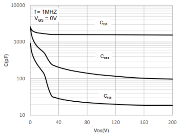
Figure 10. Capacitance Characteristics
