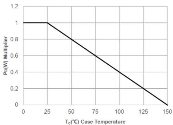
Figure 1. Power De-rating
