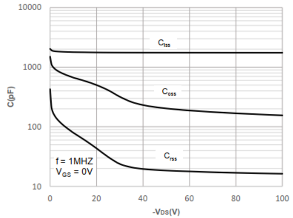
Figure 10. Capacitance Characteristics
