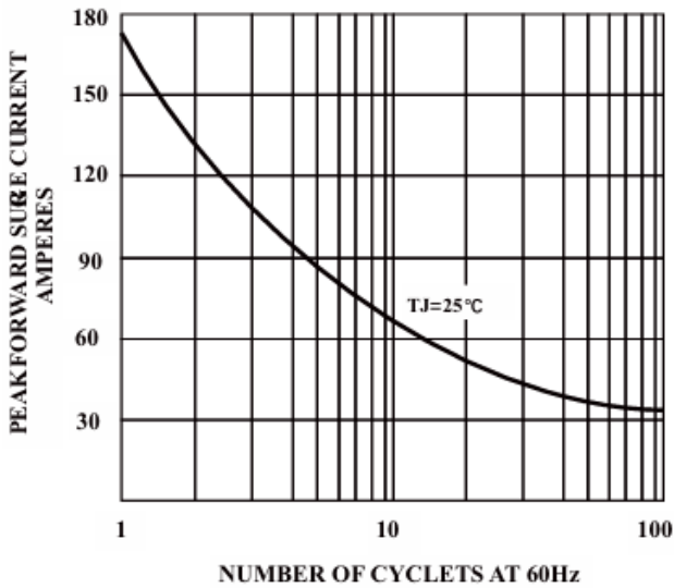
Figure 1. MAXIMUM FORWARD SURGE CURRENT
