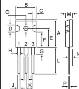
TO-3P
