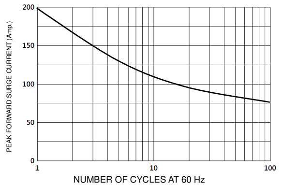
FIG-5 TYPICAL PEAK FORWARD SURGE CURRENT
