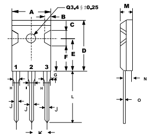
TO-247 (3P)
