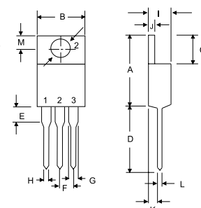
TO-220AB
