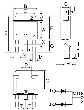
TO-252AA (D PAK)
