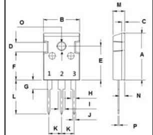
TO-3PS
