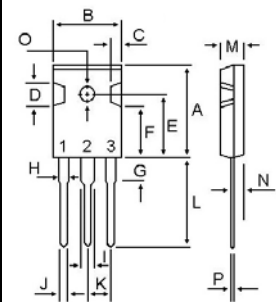
TO-3P
