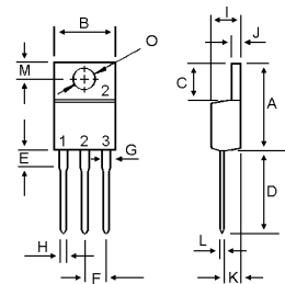
TO-220AB
