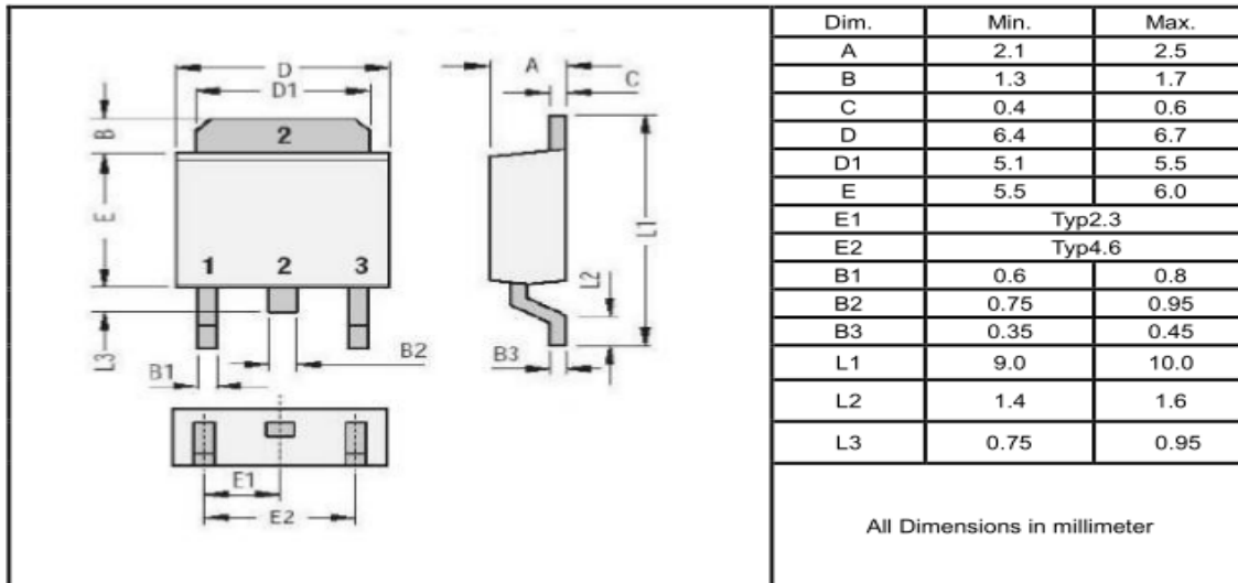
TO-252
