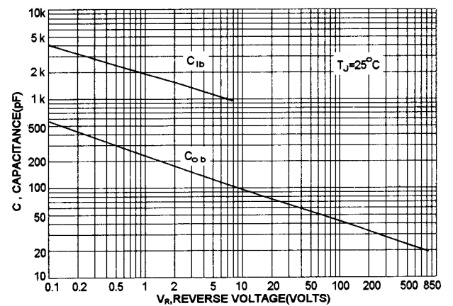
CAPACITANCE
