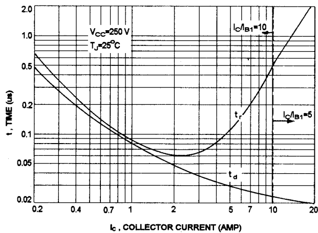
TURN-ON TIME
