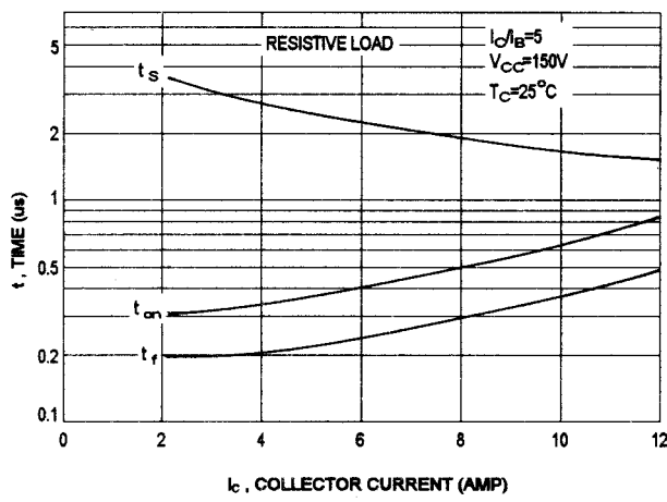
SWITCHING TIME
