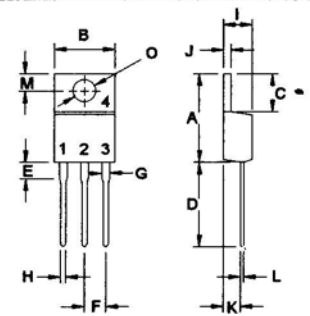
TO-220
