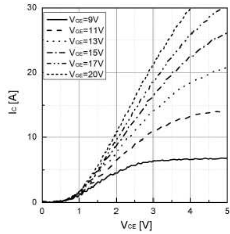
Figure 2. Typical output characteristics ( T_{vj}=150^{\circ}\text{C} )
