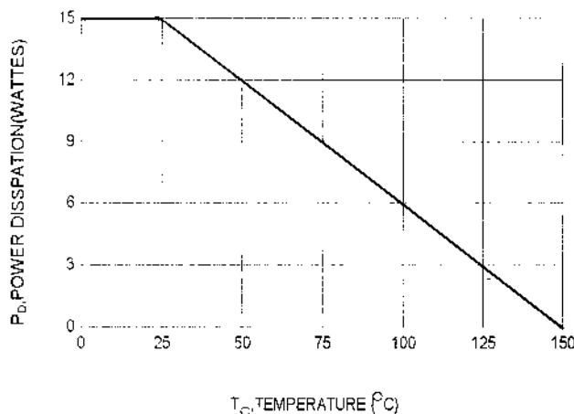
FIGURE -1 POWER DERATING
