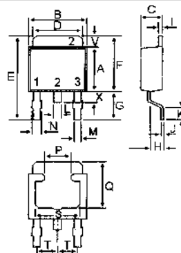
TO-252AA (DPAK)
