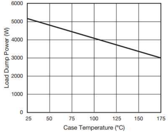
Figure 2. Load Dump Power Characteristics (10 ms Exponential Waveform)
