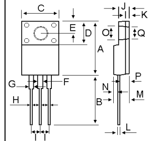
TO-220AB
